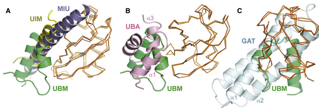
Figure 5. A Distinct Mode of Ubiquitin Recognition by UBM
