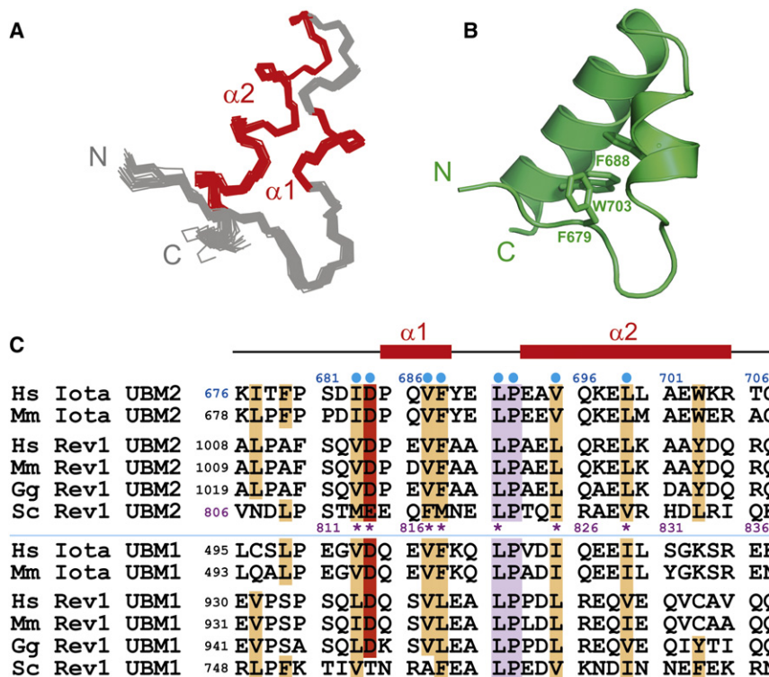
Figure 1. Structure of the Human Pol \iota UBM2
