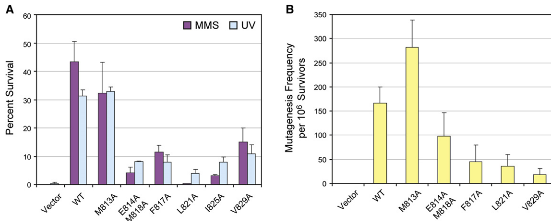
Figure 4. Mutations of Ubiquitin-Binding Residues in S. cerevisiae Rev1 UBM2 Impair REV1-Mediated Survival and Mutagenesis
