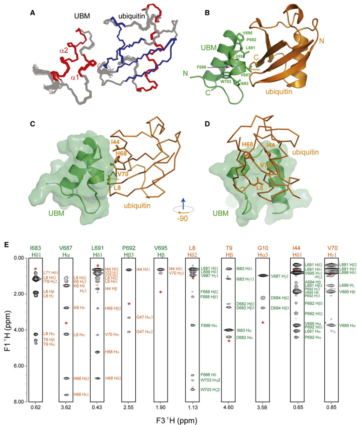
Figure 2. Structure of the Human Pol \iota UBM2-Ubiquitin Complex
