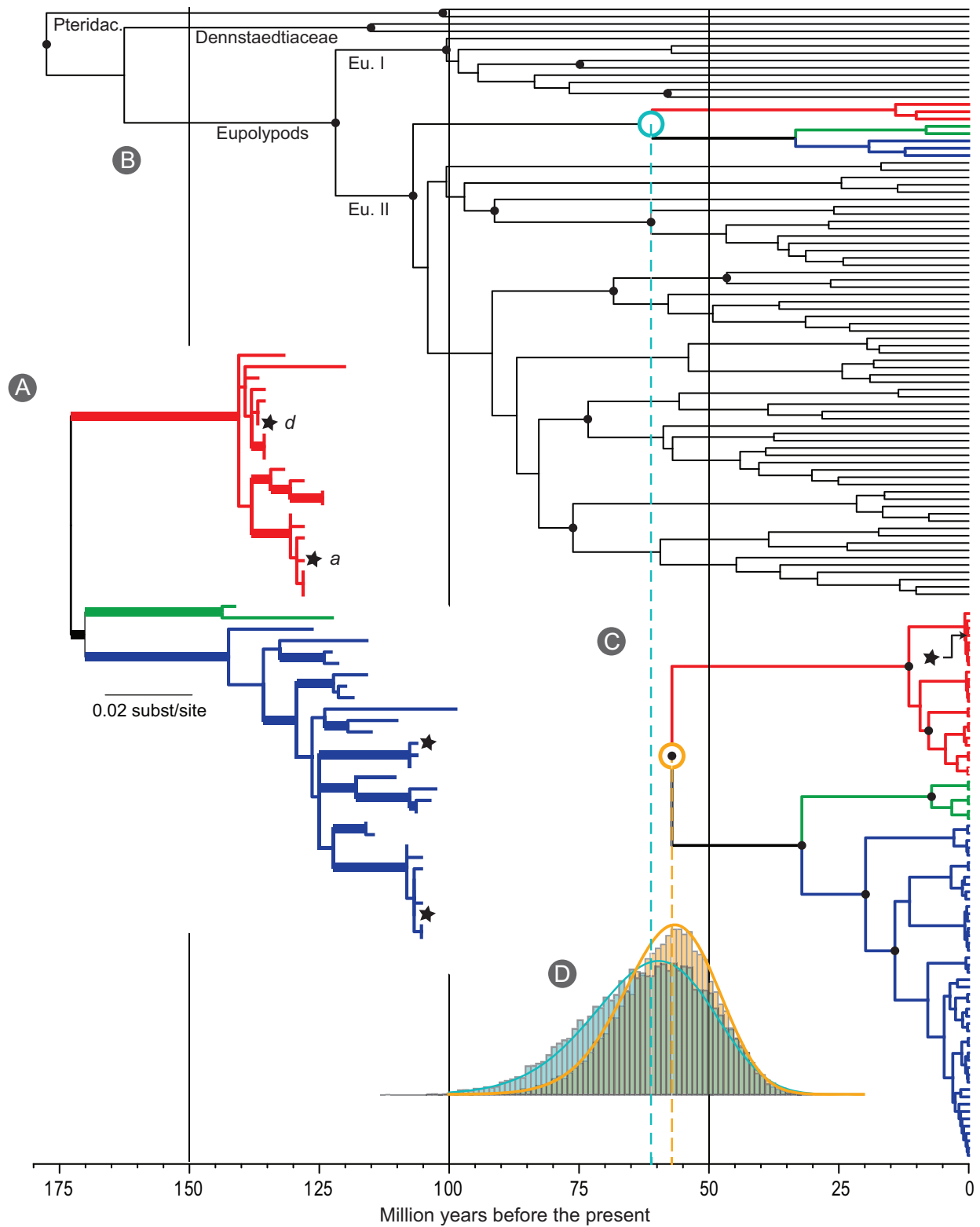
Figure 1: Evidence for the hybrid origin of x Cystocarpium and a sequential empirical Bayesian analysis of divergence time. A , Maximum likelihood phylogram of nuclear gapCp data; thickened branches have \geq 70\% bootstrap support; “a” and “d” indicate, respectively, the
