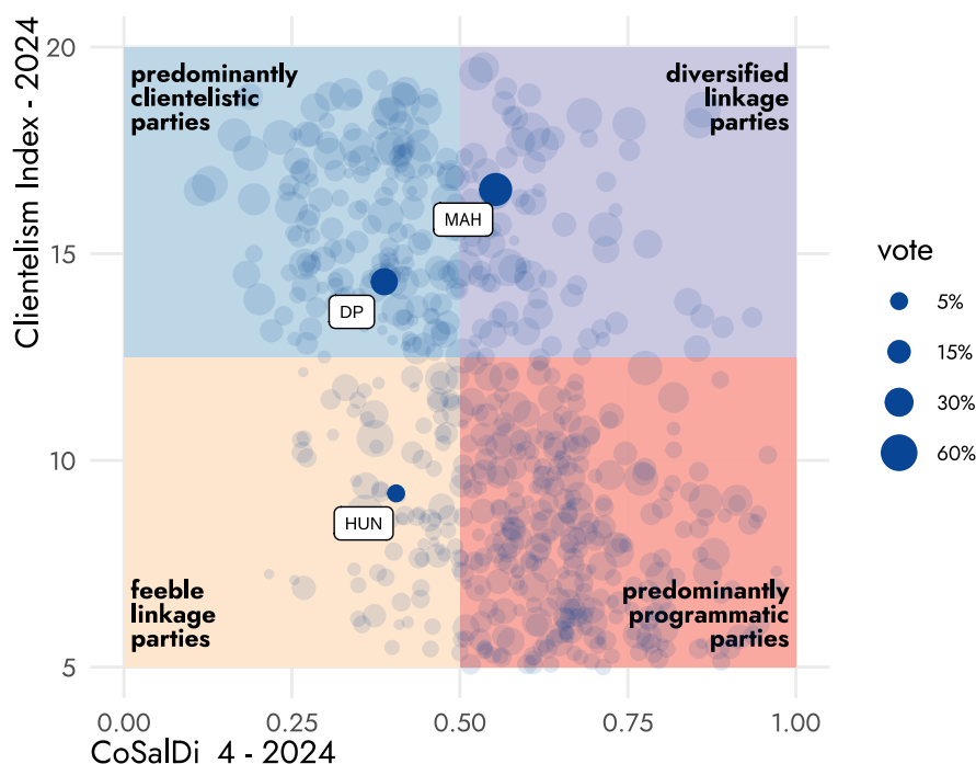
Figure 9: Just Clientelism and Programmatism: How Sharp is the Trade-off in Mongolia? (2024 DALP II B15 X Cosaldi_4)
