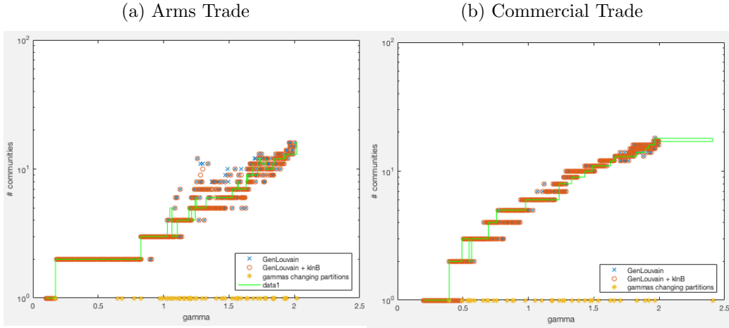
Figure A.2: Resolution Parameter Searches for Robust Gamma Values
