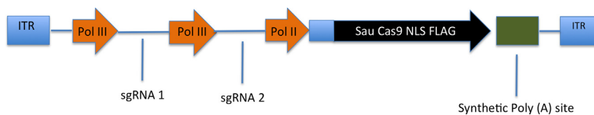
Fig. 2. A potential AAV multiplex Cas9 delivery vector. The minimal Cas9 protein from S. aureus has a total coding size of \sim 3.2 kb, including an epitope tag and an NLS, and this shorter Cas9 enzyme therefore opens up substantial packaging space in AAV. Minimal Pol II and Pol III promoters and a synthetic Poly A sequence can be employed to minimize the nucleotide footprints of these cis-elements. In total, we have now generated small AAV-based CRISPR/Cas9 expression vectors that encode both the Sau Cas9 protein and two independent sgRNAs yet occupy < 4.5 kb of packaging space, well below the AAV size limit of \sim 4.7 kb.
